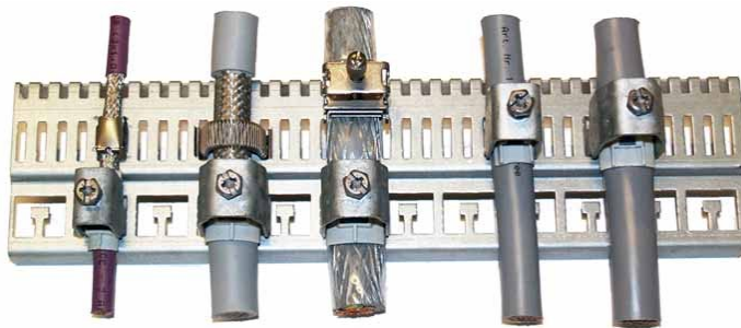
Figure 7: Examples of the Earthing of the Cable Screening
