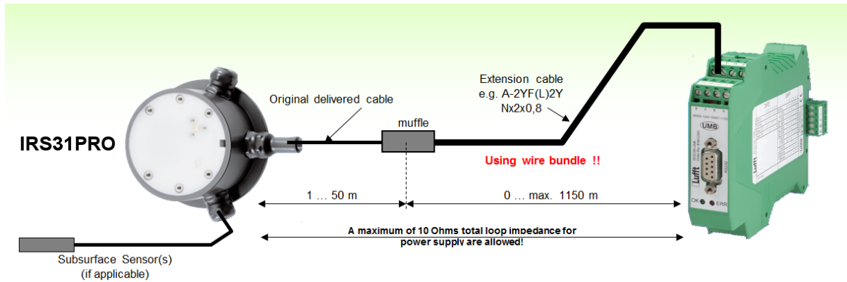
Figure 4: Cable Extension
