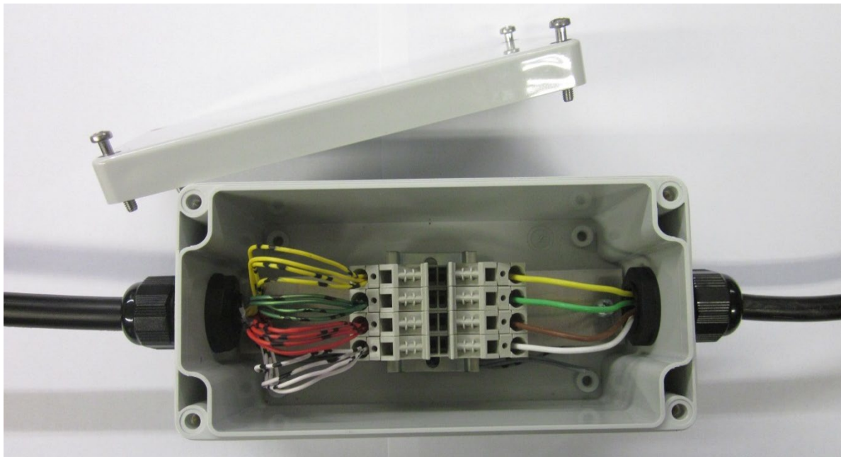
Figure 5: Example of an Extension Box
