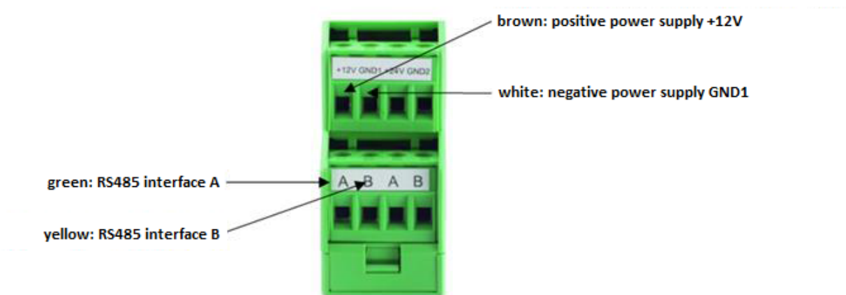
Figure 8: ISOCON-UMB Connection
